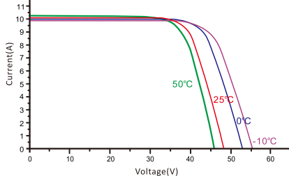
I-V characteristics at different temperatures (AM1.5, 1000W/m²)
